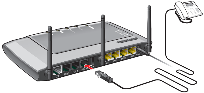
Connecting an ISDN telephone to the FRITZ!Box
